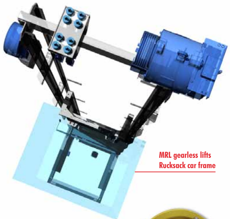
MRL gearless lifts Rucksack car frame
